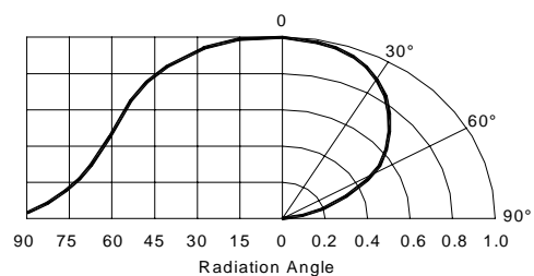
Typical Radiation Pattern 120°
